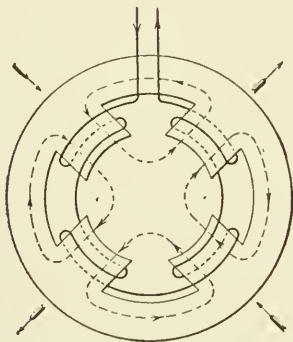
Fig. 133. Motor Field Coils Properly Wound
